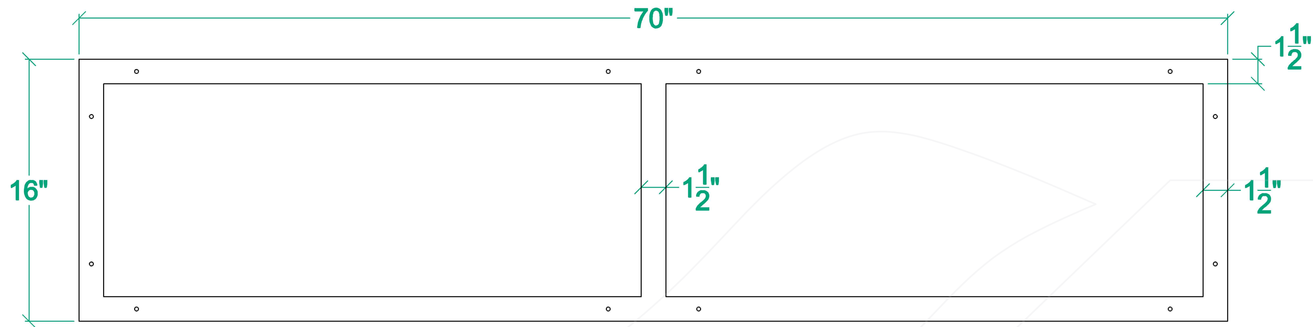
TOP VIEW
