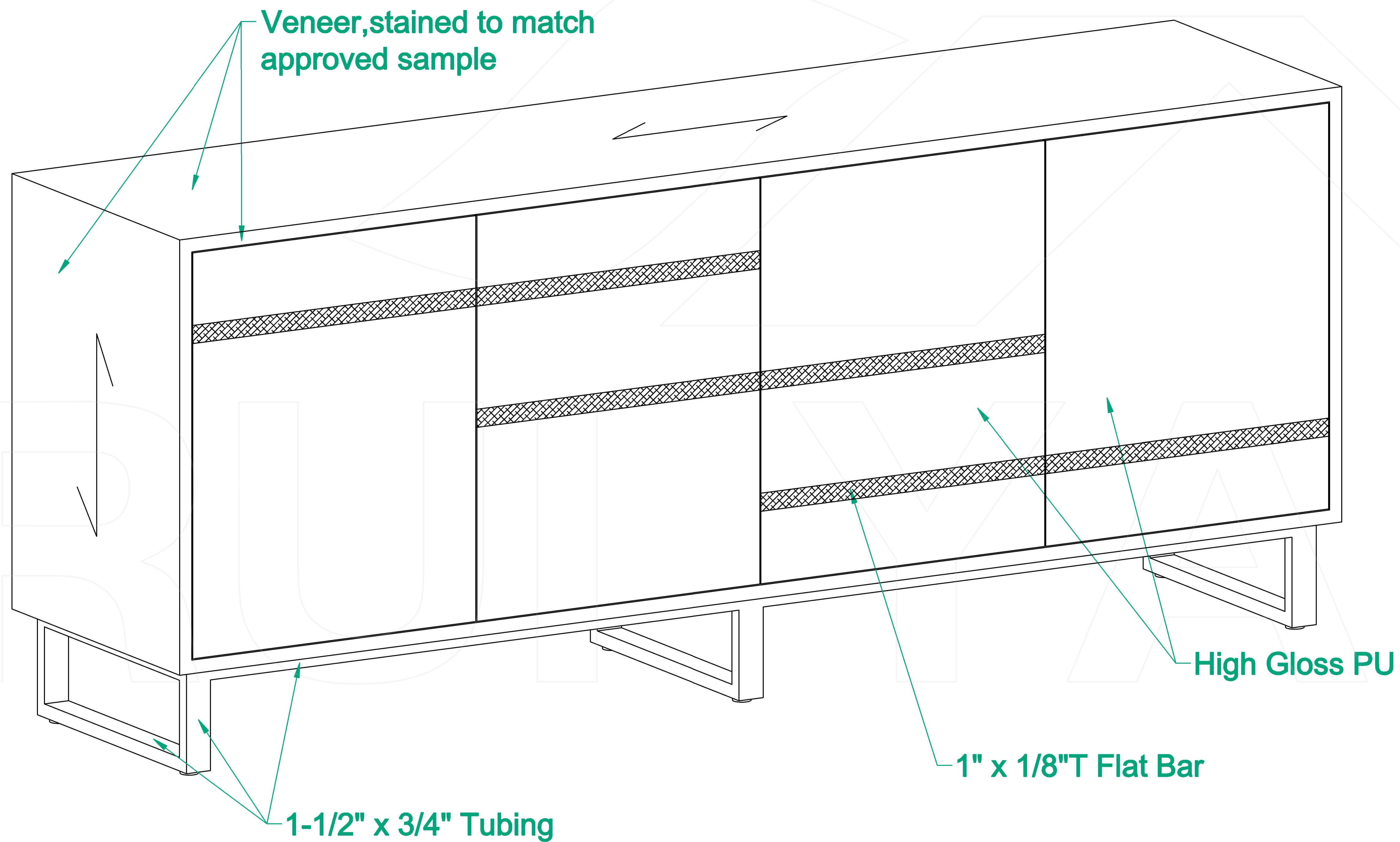
ISOMETRIC VIEW
