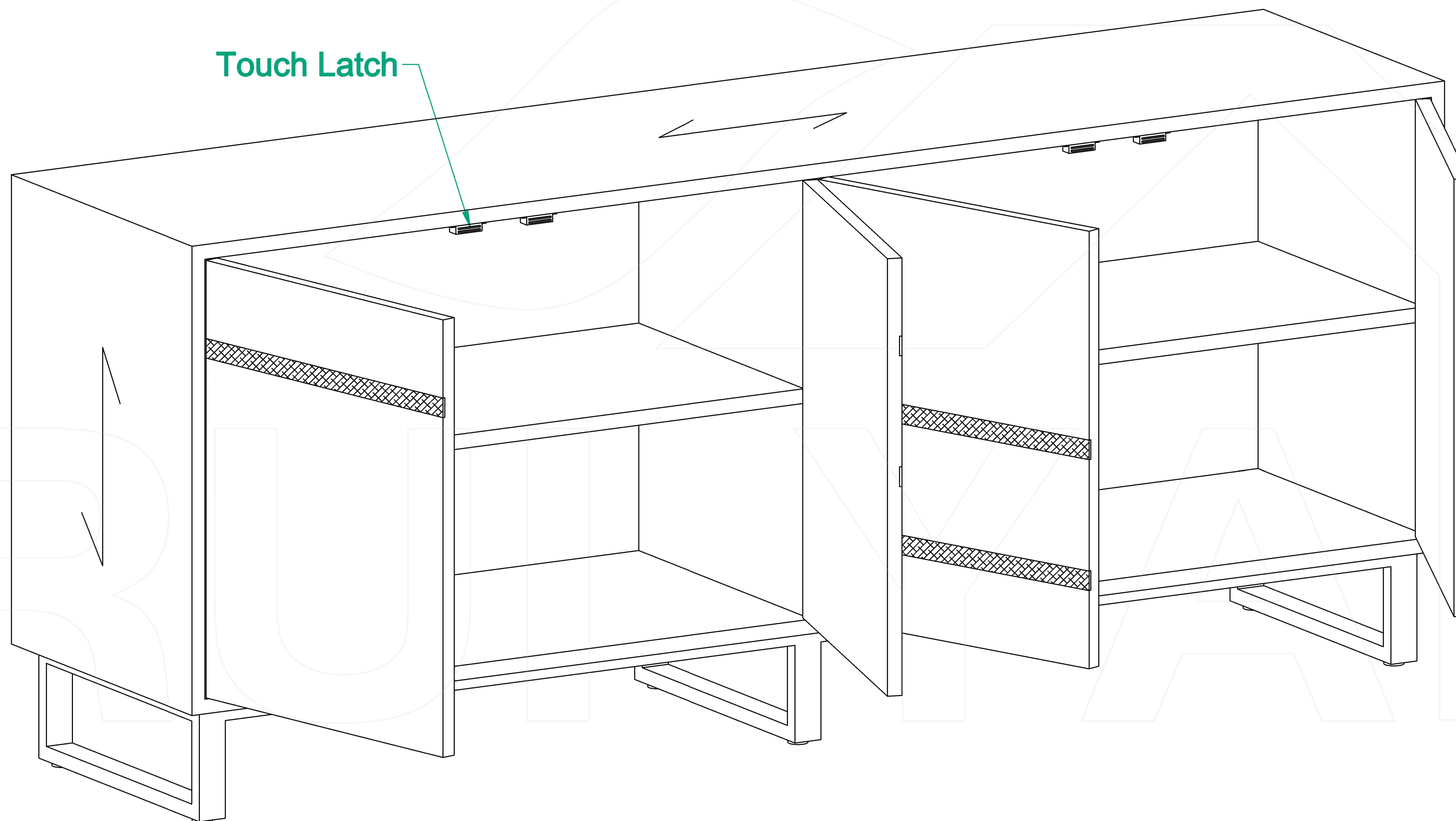
ISOMETRIC VIEW
